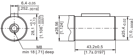
CO - \phi 1" straight, Parallel key \frac{1}{4} \times \frac{1}{4} \times 1\frac{1}{4} BS46 Max. Torque 34 daNm [3010 lb-in]
