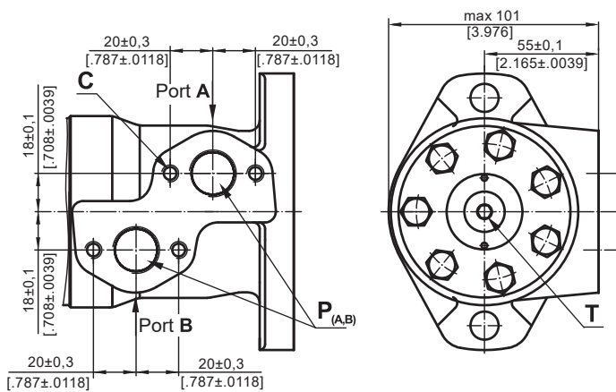
Side Ports
